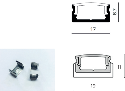
Bracket detail
