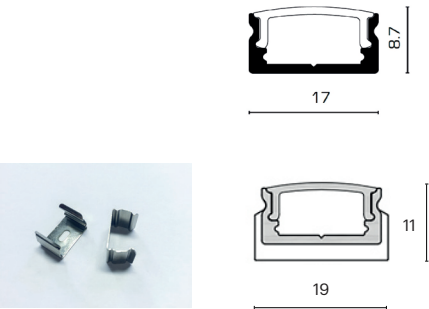
Bracket detail
