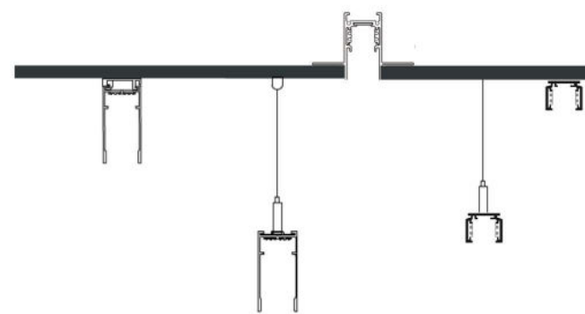
Suspended, Surface &amp; Recessed
