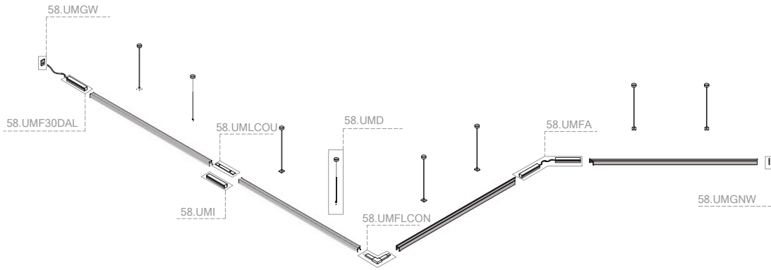
Profile 58.UMA2M High Suspended
